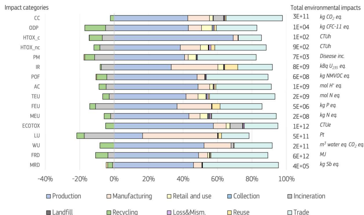
Figure 9. Life cycle impacts of the whole 2022 EU plastic value chain and percentage contribution to 100% of each impact category and life cycle stage. The same legend applies to all bar charts.
